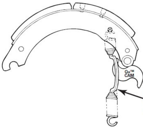
OFFSET RETURN SPRING (MERITOR PART 2258Y1273)
